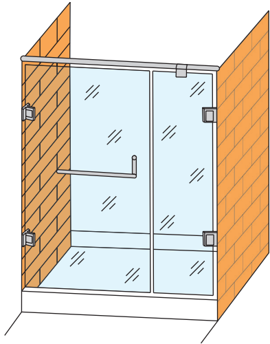
Parede/vidro 90° Glass to wall 90° Mur/verre 90° Pared/cristal 90°
